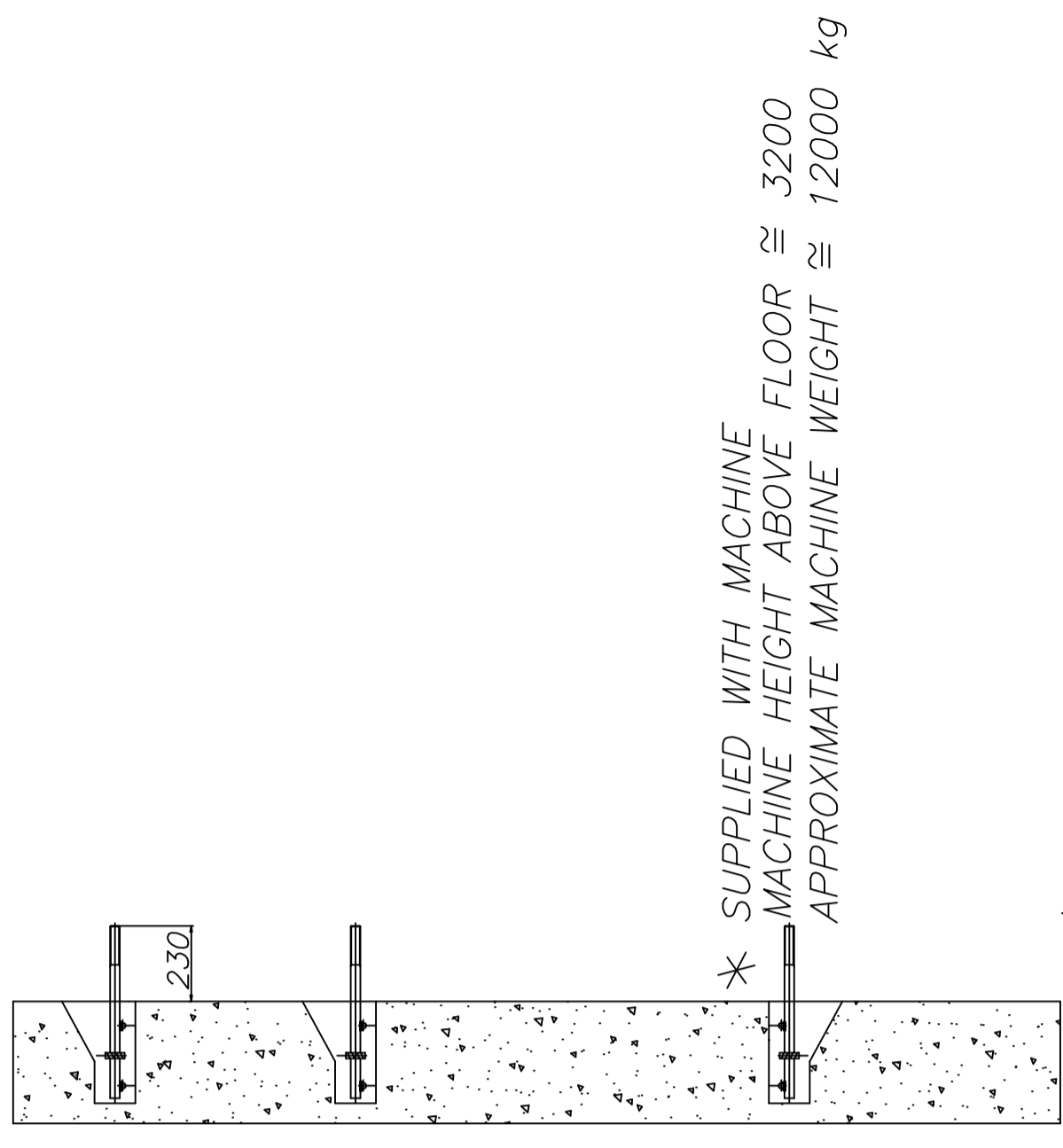
Section B-B
